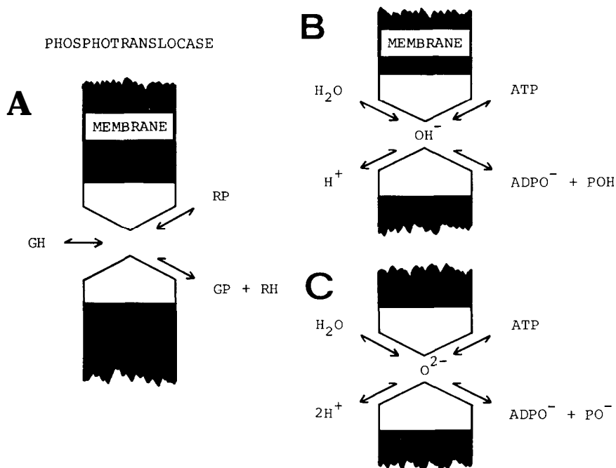
Fig. 9. Topologically macroscopic chemiosmotic group conduction: A, of group G, energised by phosphate transfer; B and C, of OH - and O 2- respectively, energised by ATP hydrolysis.
