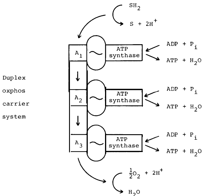
Fig. 3. Phosphorylating respiratory chain: Local interaction coupling hypothesis. The symbol \sim represents a localised "high-energy" chemical intermediary or physical state.
