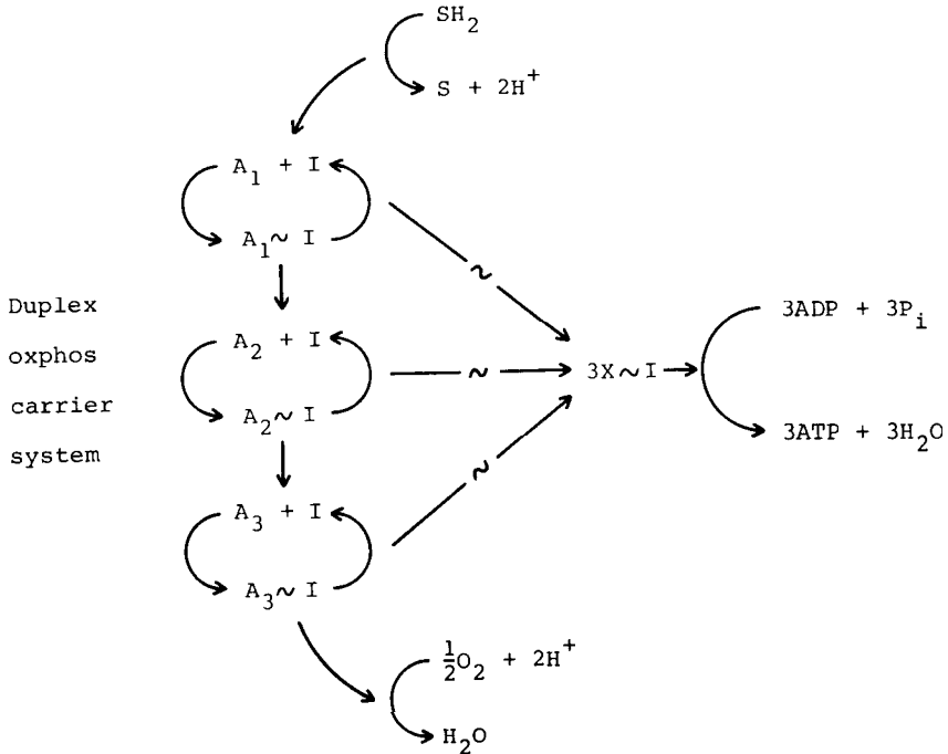
Fig. 2. Phosphorylating respiratory chain: Chemical coupling hypothesis. \text{A} \sim \text{I} and \text{X} \sim \text{I} represent hypothetical high-energy chemical intermediates; and the symbol \sim represents the so-called high-energy bond.
