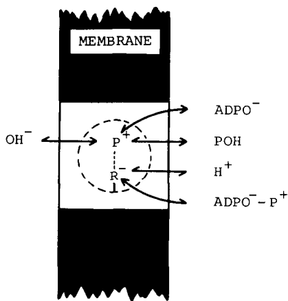
Fig. 10. Protonmotive ATPase translocating OH - (from Mitchell, 1961c).
